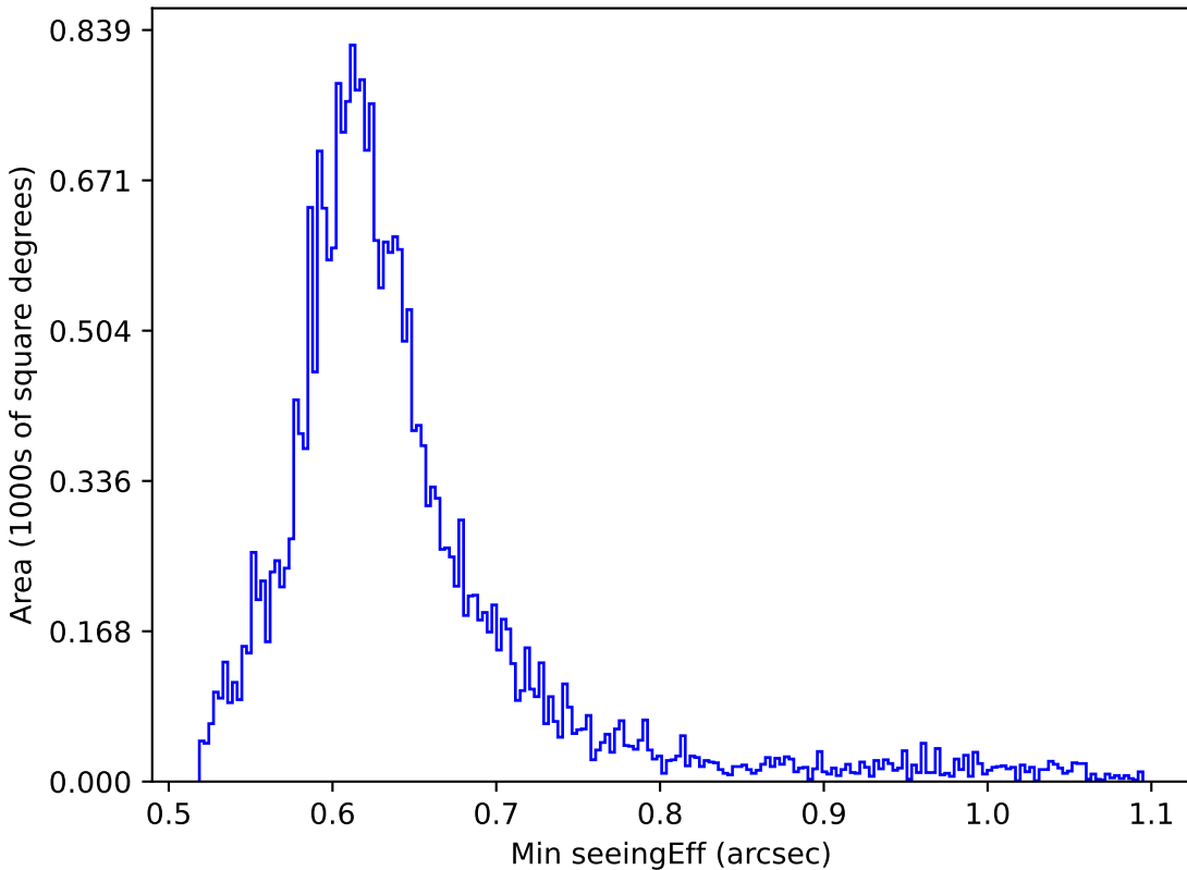
no_high_blob_v3.3_10yrs All sky r band: Min seeingEff
