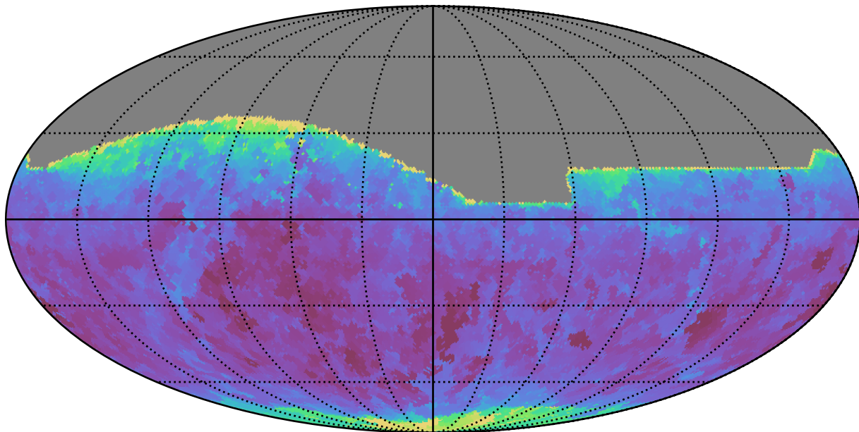
no_high_blob_v3.3_10yrs All sky i band: Min seeingEff
