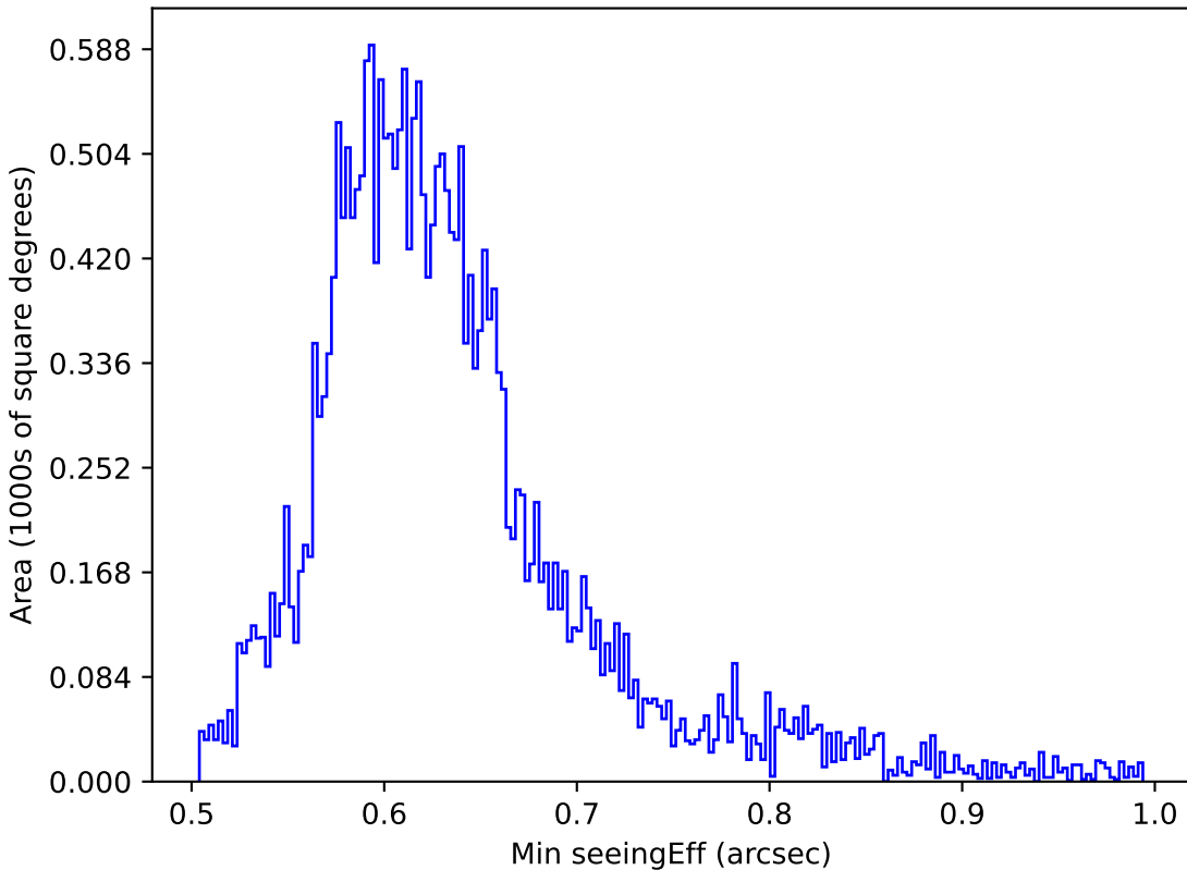
no_high_blob_v3.3_10yrs All sky i band: Min seeingEff
