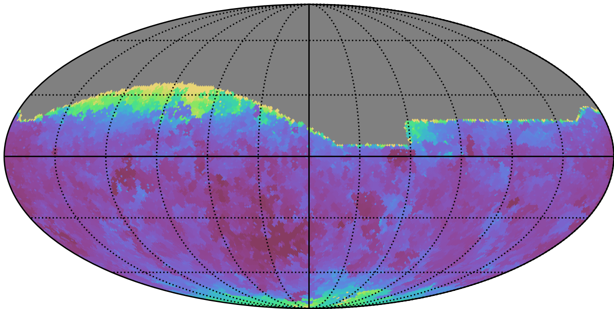
no_high_blob_v3.3_10yrs All sky g band: Min seeingEff
