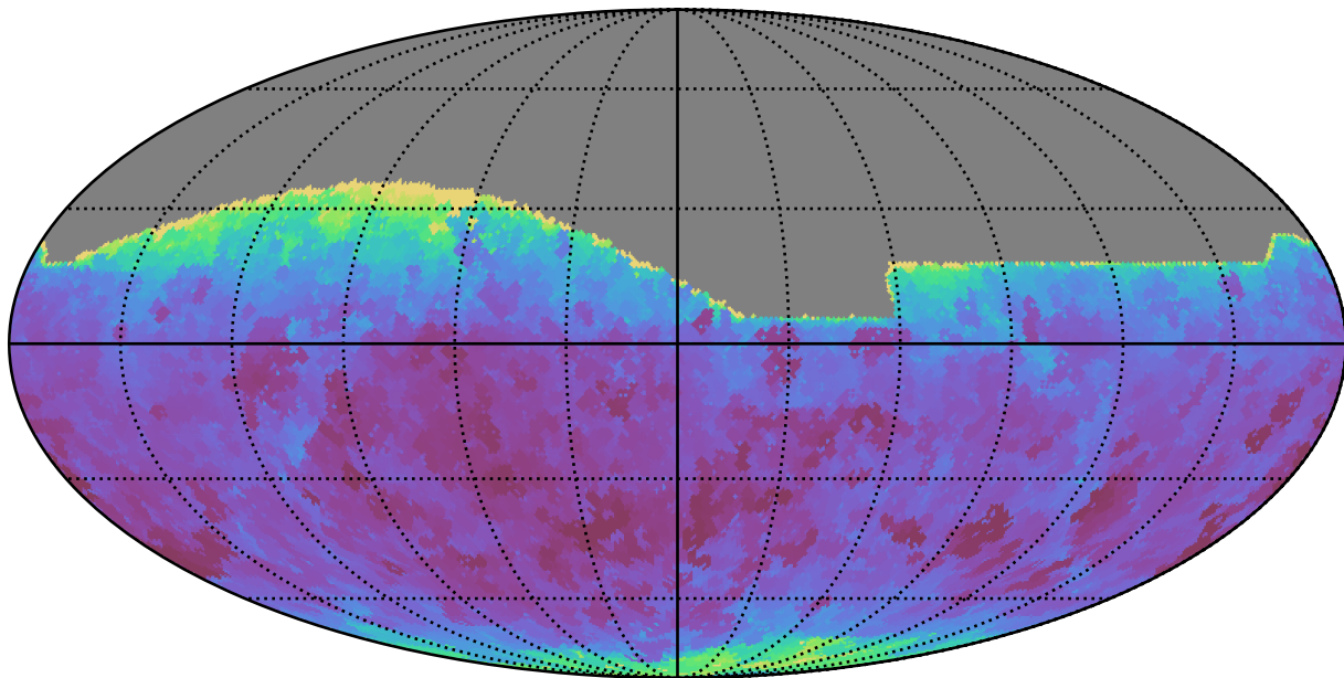
no_high_blob_v3.3_10yrs All sky all bands: Min seeingEff
