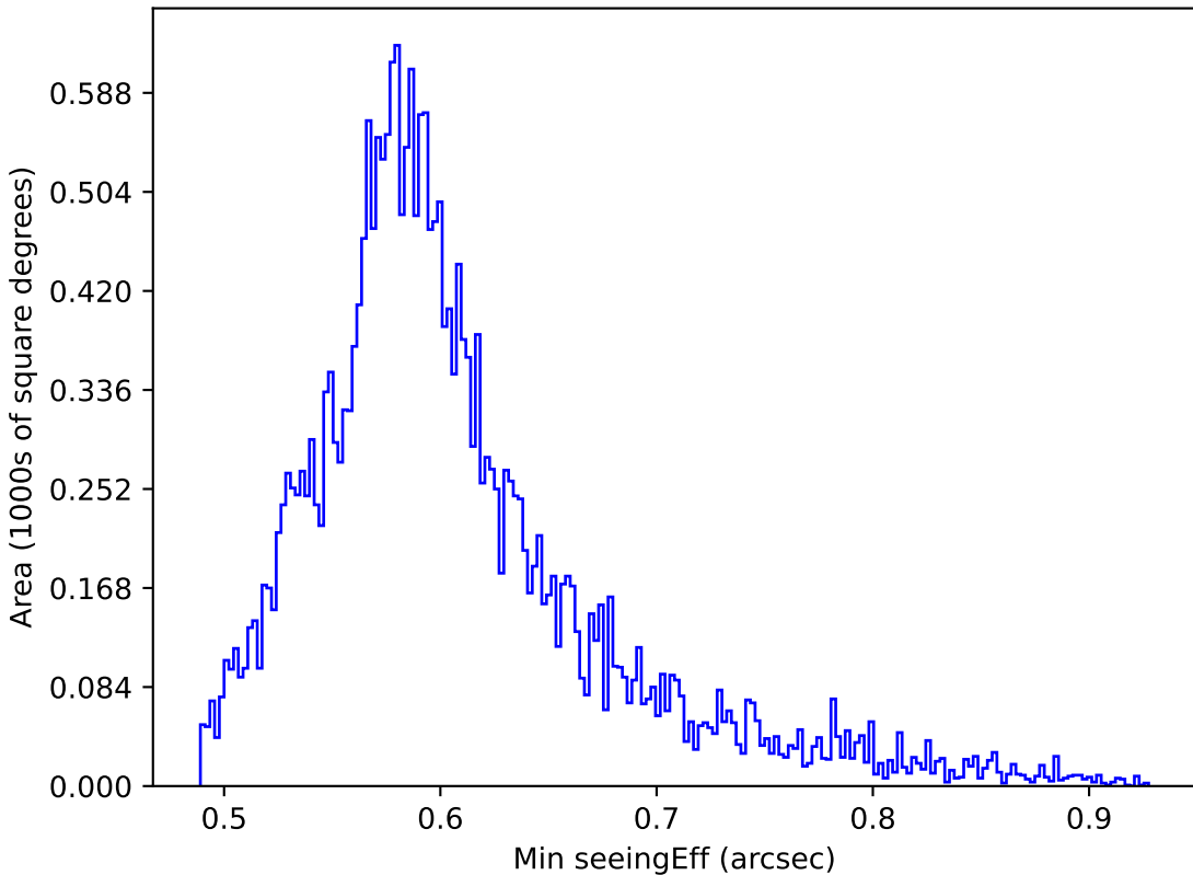
no_high_blob_v3.3_10yrs All sky all bands: Min seeingEff
