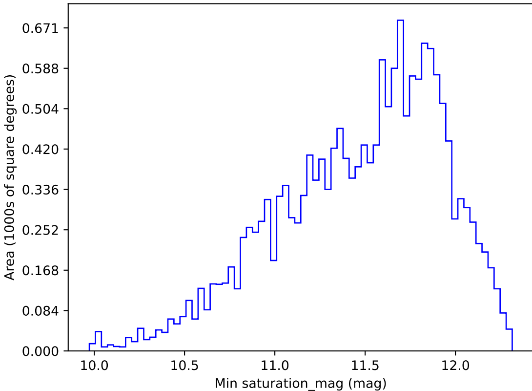
no_high_blob_v3.3_10yrs WFD u band: Min saturation_mag
