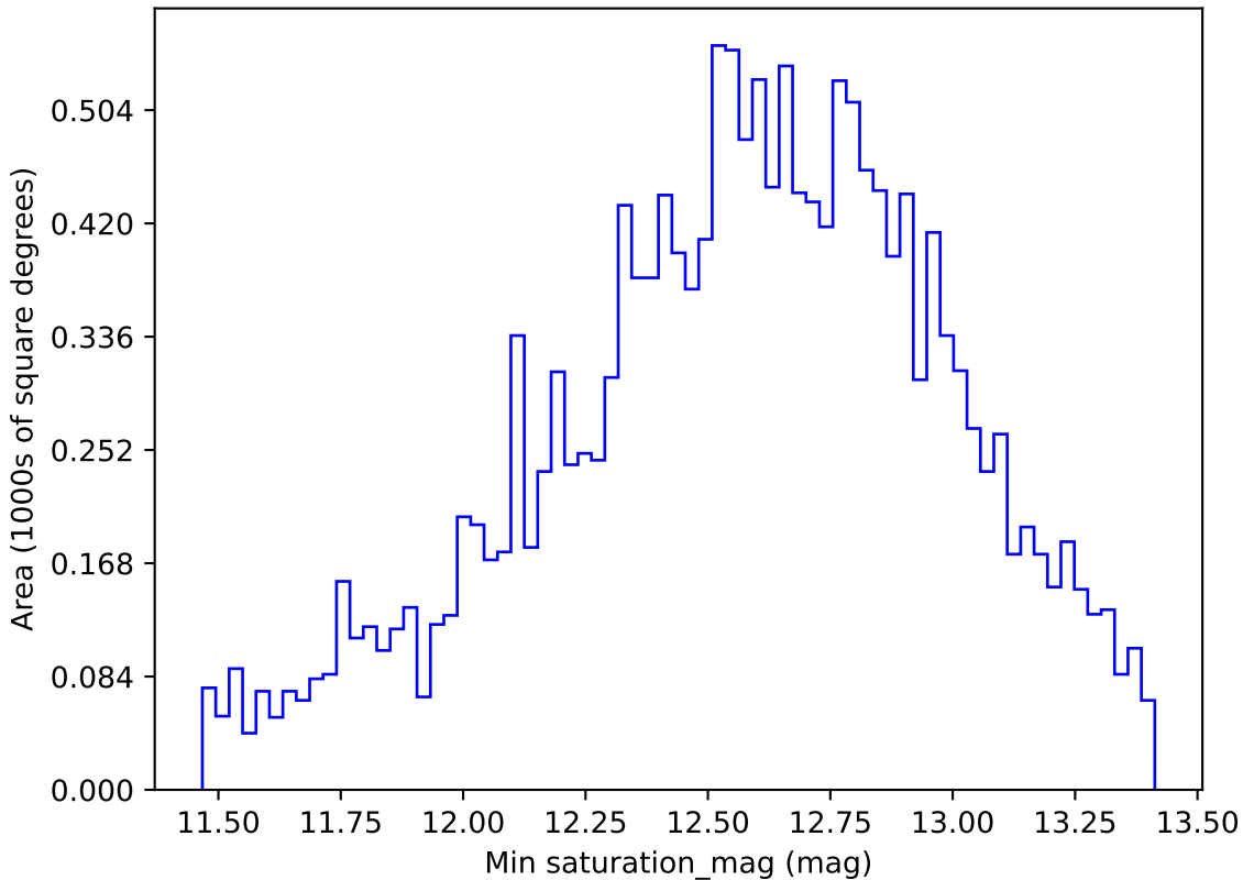
no_high_blob_v3.3_10yrs WFD r band: Min saturation_mag
