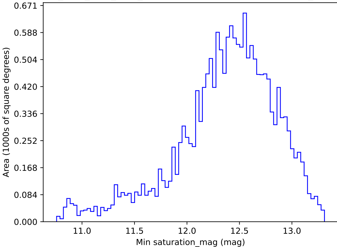
no_high_blob_v3.3_10yrs WFD i band: Min saturation_mag
