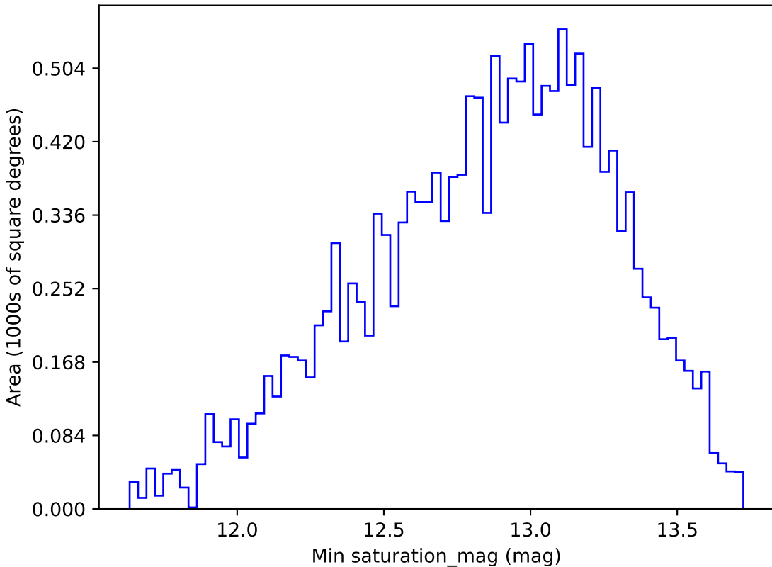
no_high_blob_v3.3_10yrs WFD g band: Min saturation_mag
