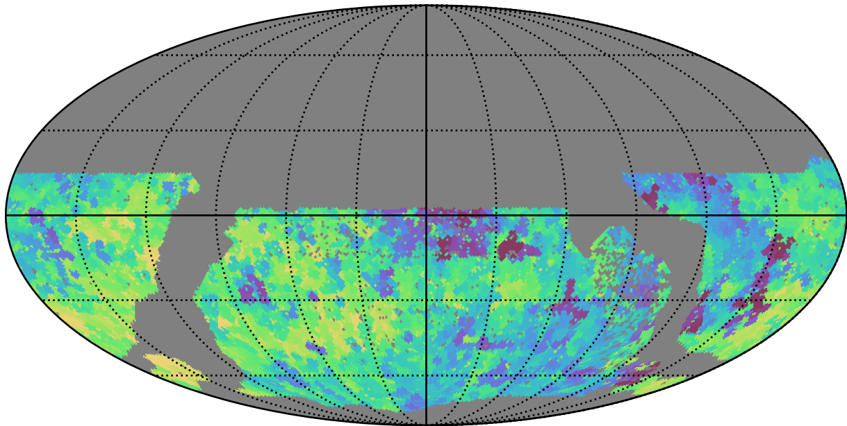
no_high_blob_v3.3_10yrs WFD all bands: Min saturation_mag
