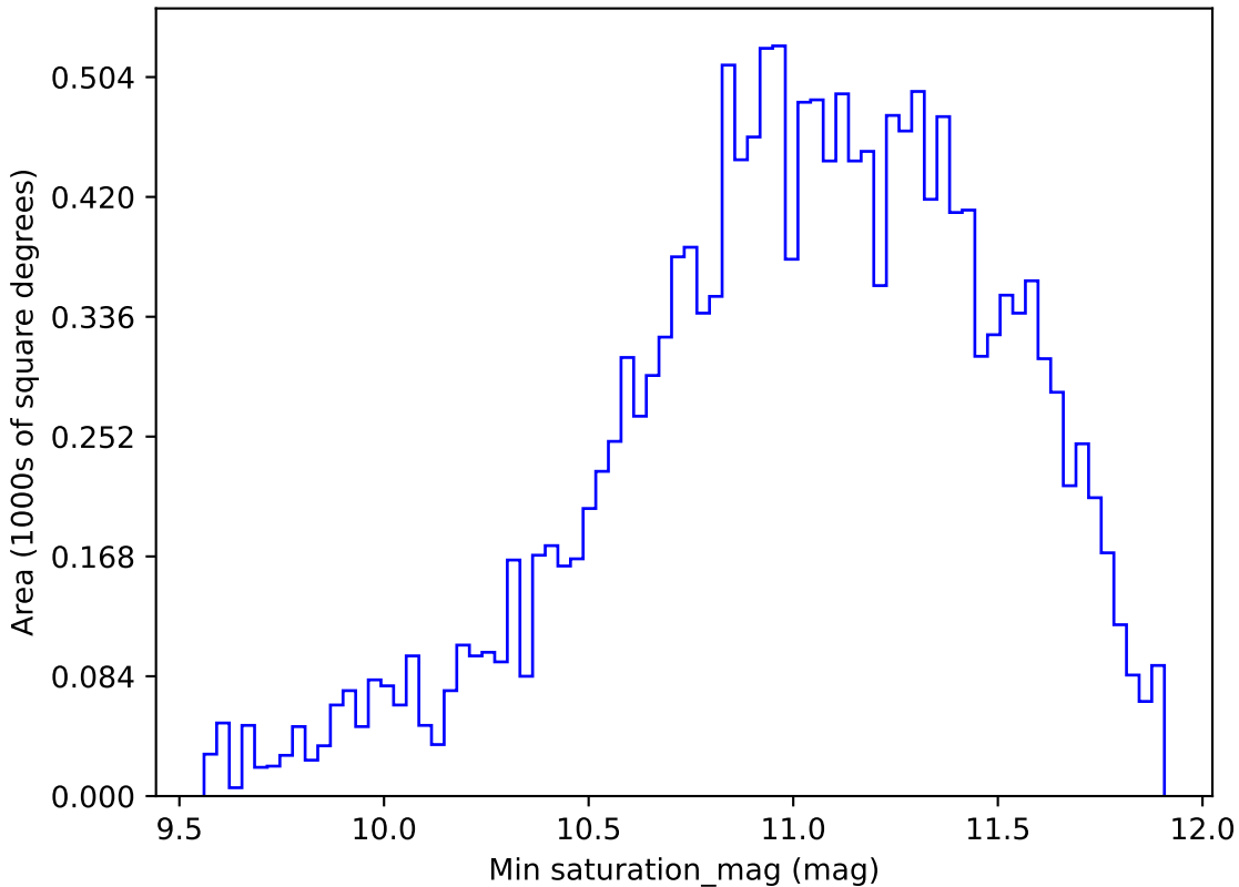
no_high_blob_v3.3_10yrs WFD all bands: Min saturation_mag
