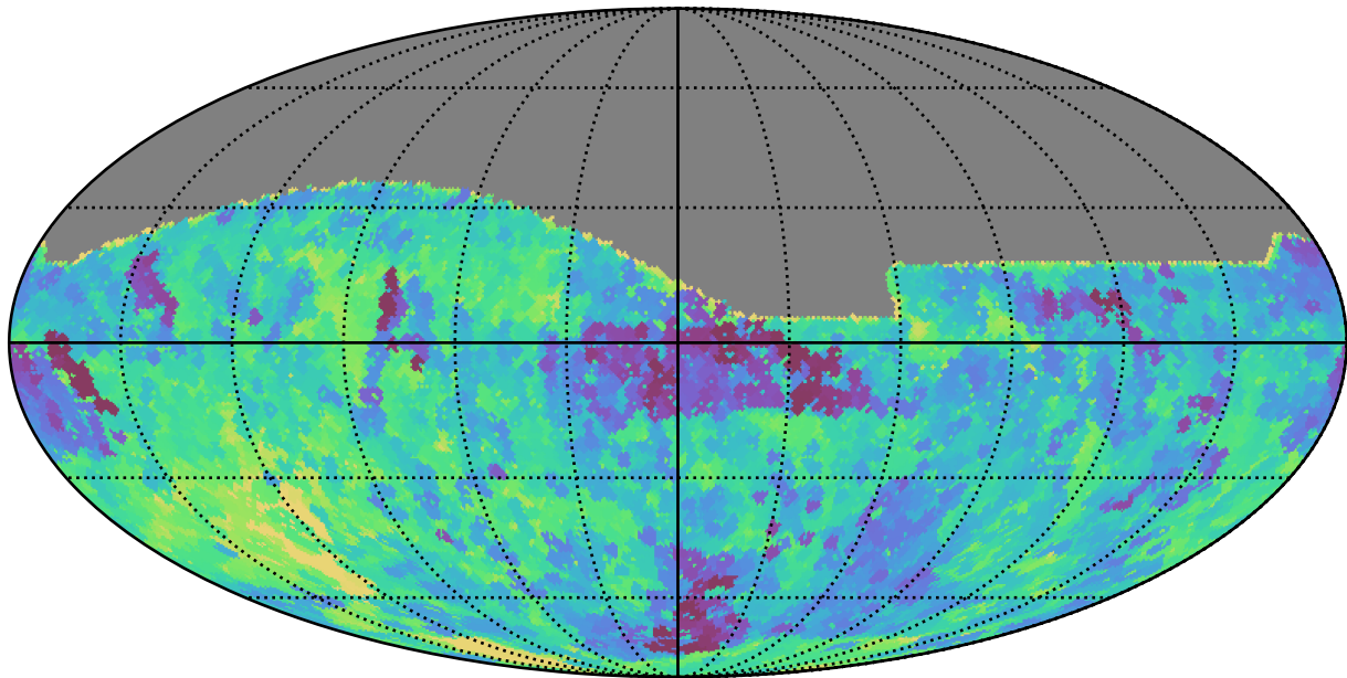
no_high_blob_v3.3_10yrs All sky z band: Min saturation_mag
