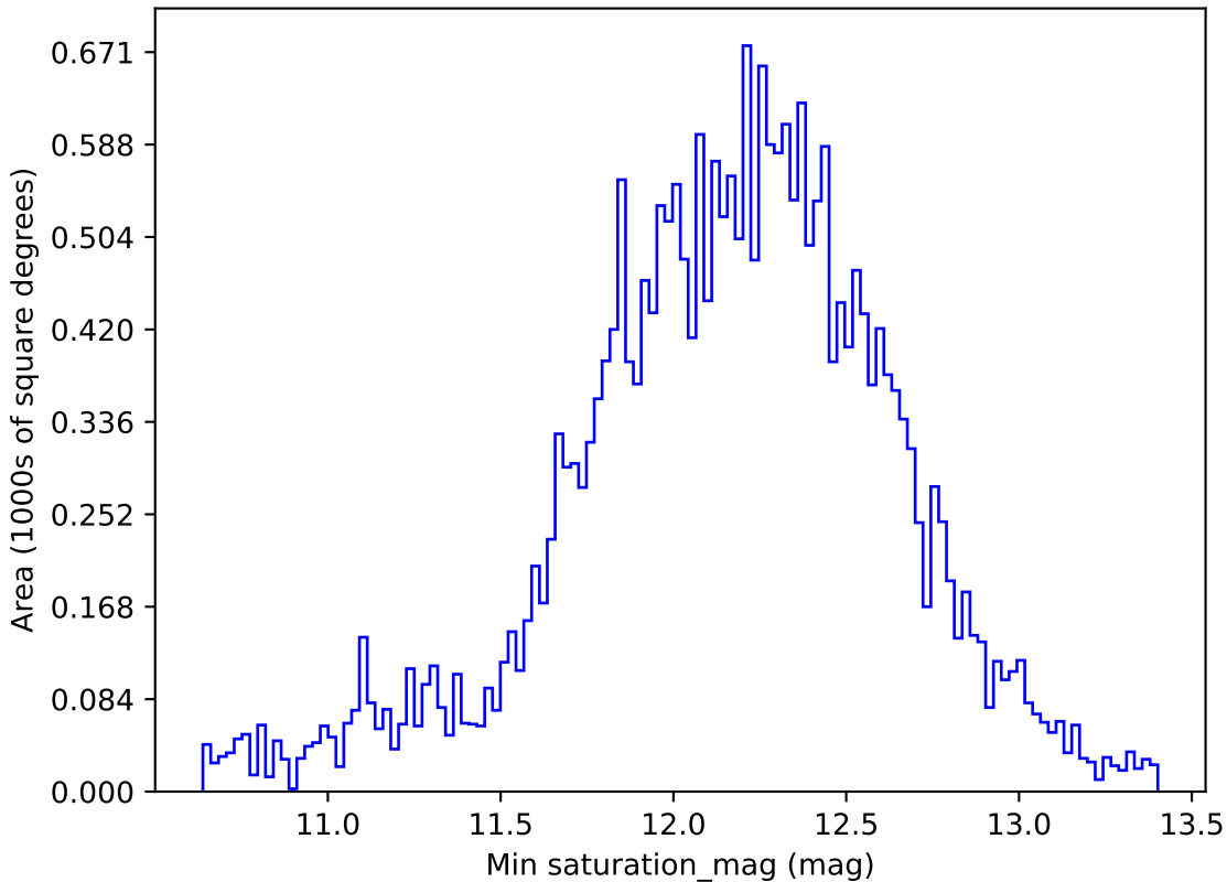
no_high_blob_v3.3_10yrs All sky z band: Min saturation_mag
