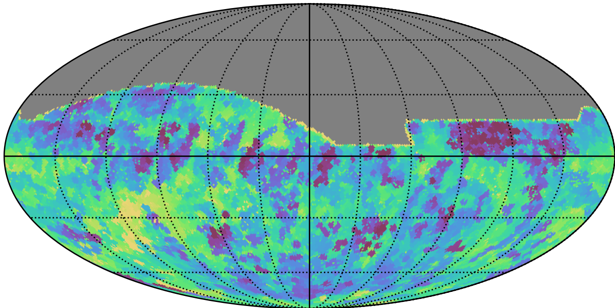
no_high_blob_v3.3_10yrs All sky r band: Min saturation_mag
