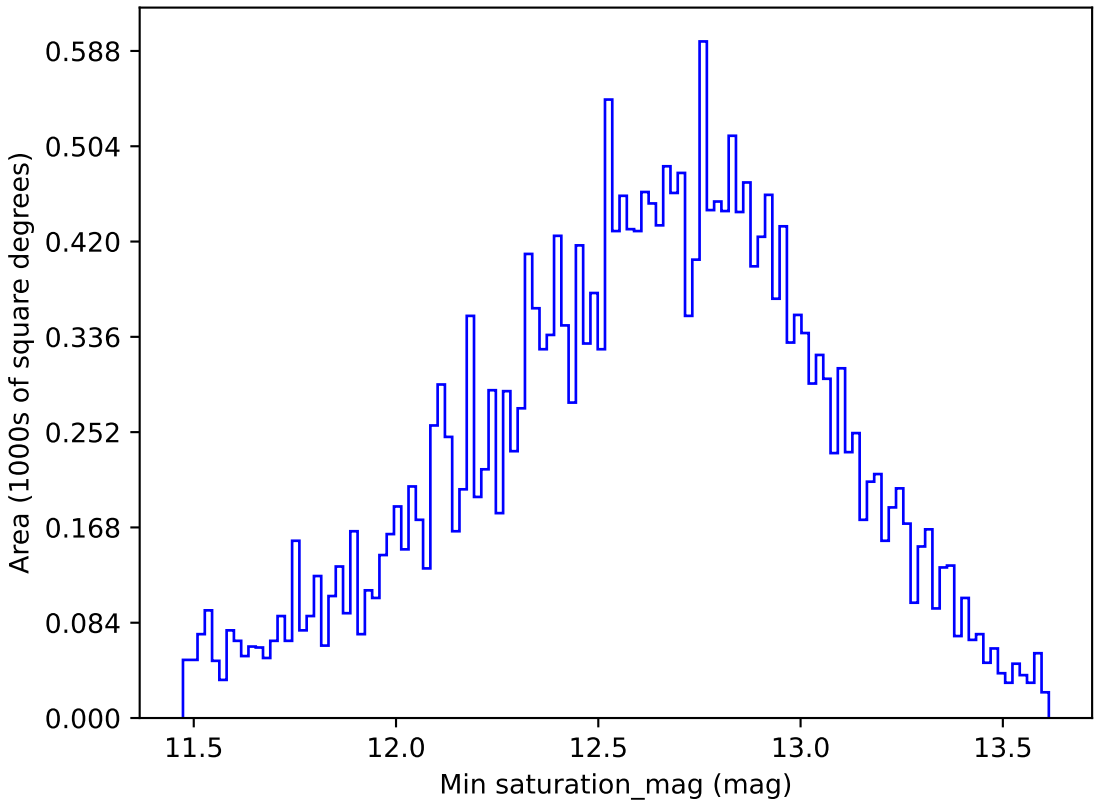
no_high_blob_v3.3_10yrs All sky r band: Min saturation_mag
