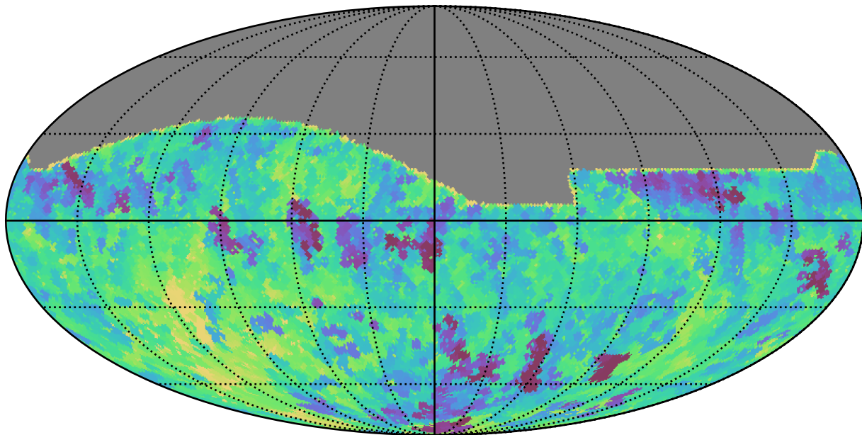
no_high_blob_v3.3_10yrs All sky i band: Min saturation_mag
