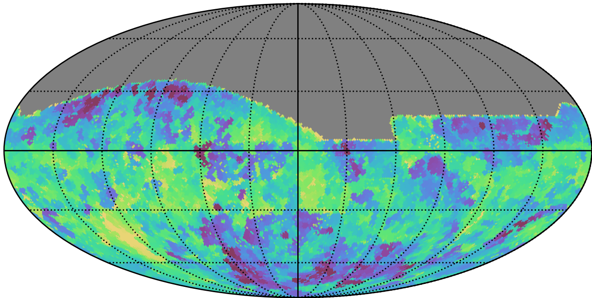
no_high_blob_v3.3_10yrs All sky g band: Min saturation_mag
