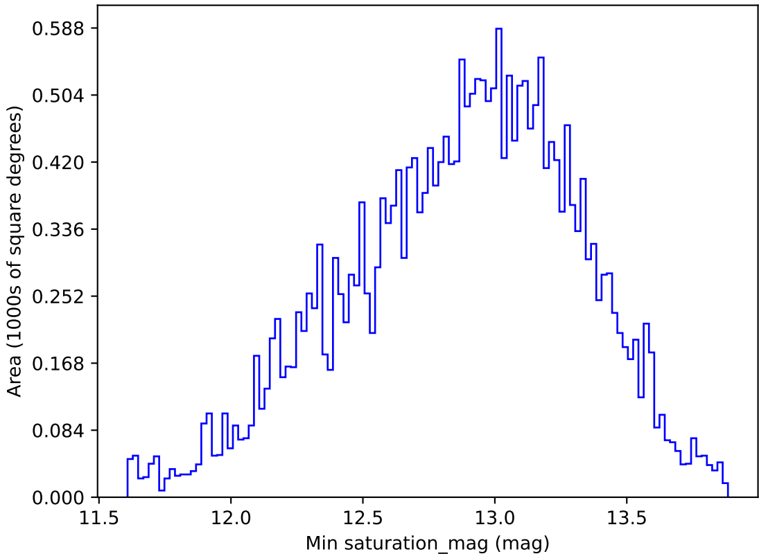
no_high_blob_v3.3_10yrs All sky g band: Min saturation_mag
