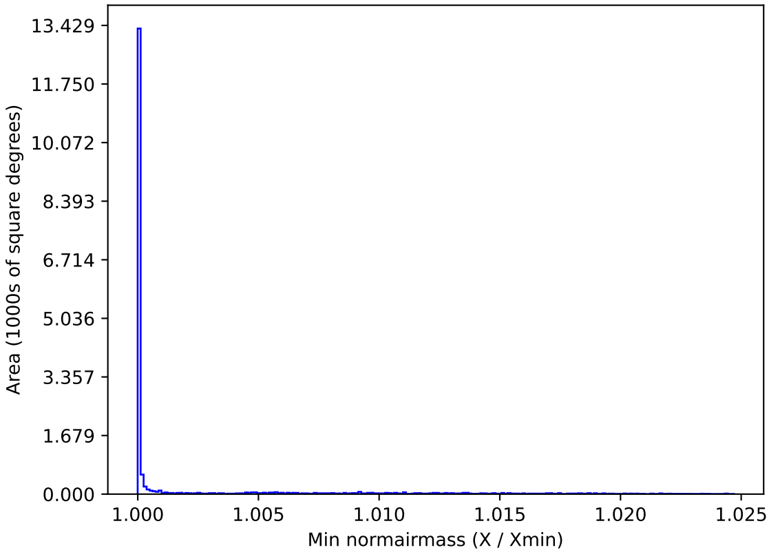
no_high_blob_v3.3_10yrs WFD z band: Min normairmass
