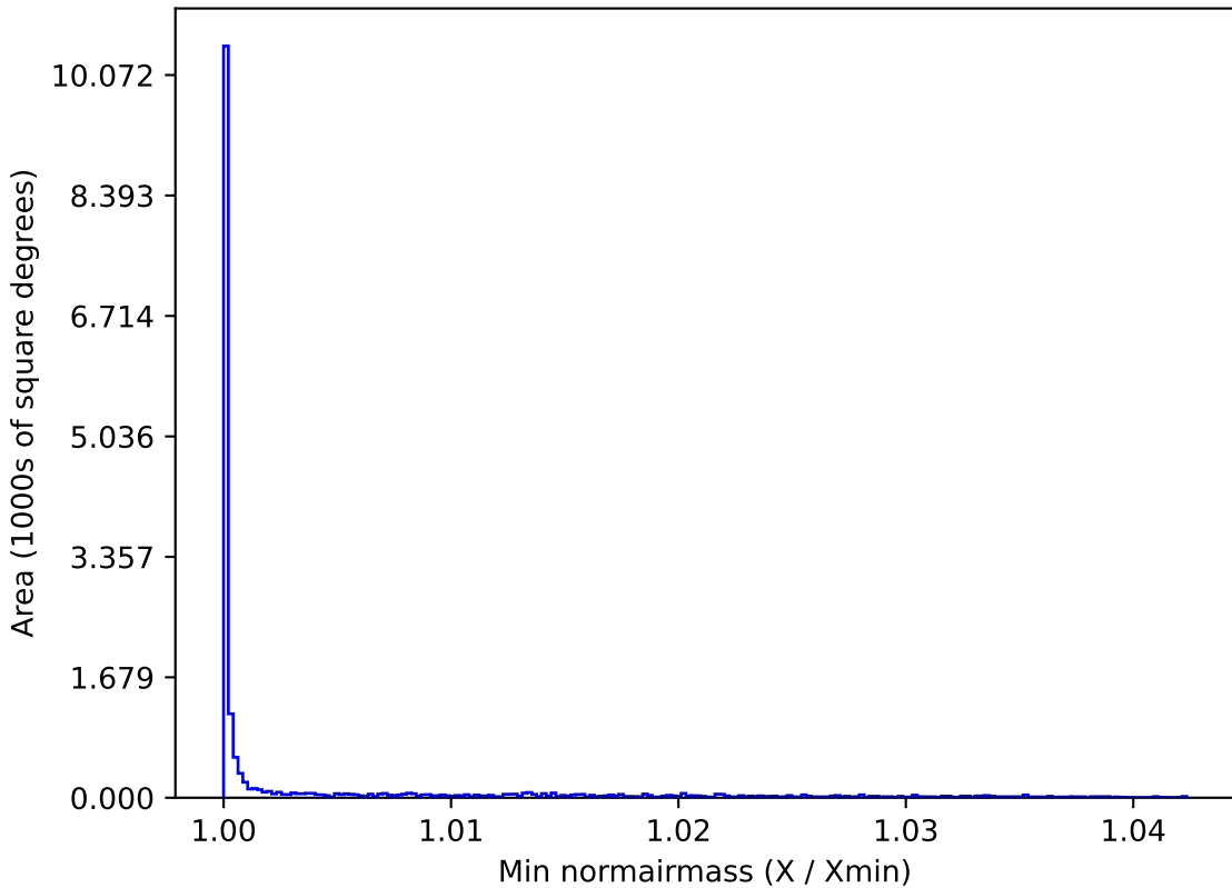
no_high_blob_v3.3_10yrs WFD u band: Min normairmass
