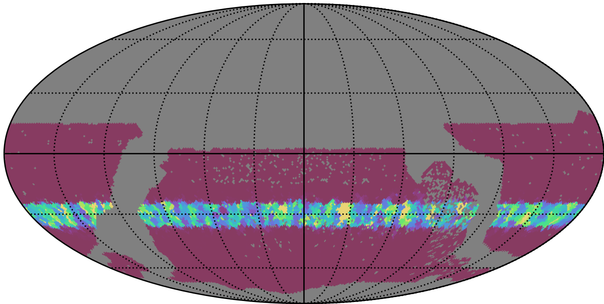
no_high_blob_v3.3_10yrs WFD i band: Min normairmass
