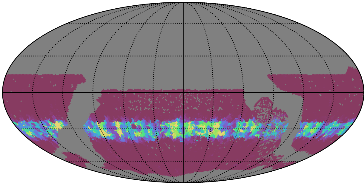
no_high_blob_v3.3_10yrs WFD g band: Min normairmass
