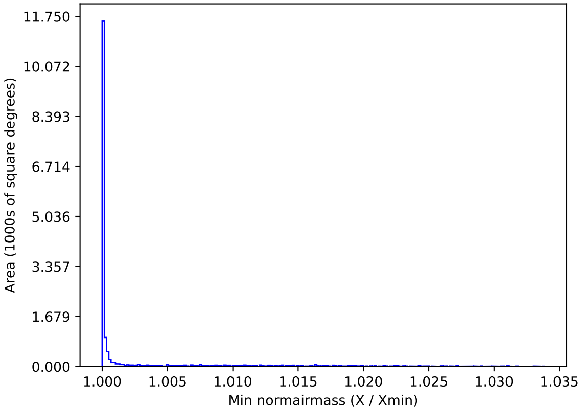
no_high_blob_v3.3_10yrs WFD g band: Min normairmass
