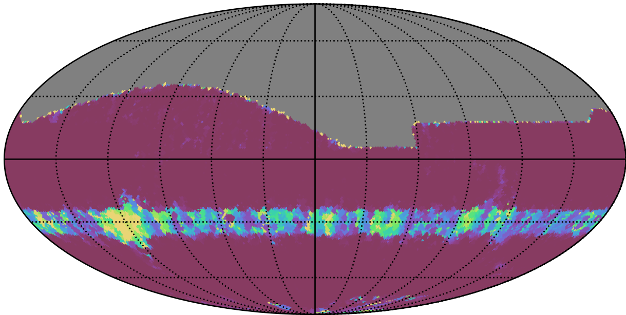
no_high_blob_v3.3_10yrs All sky z band: Min normairmass
