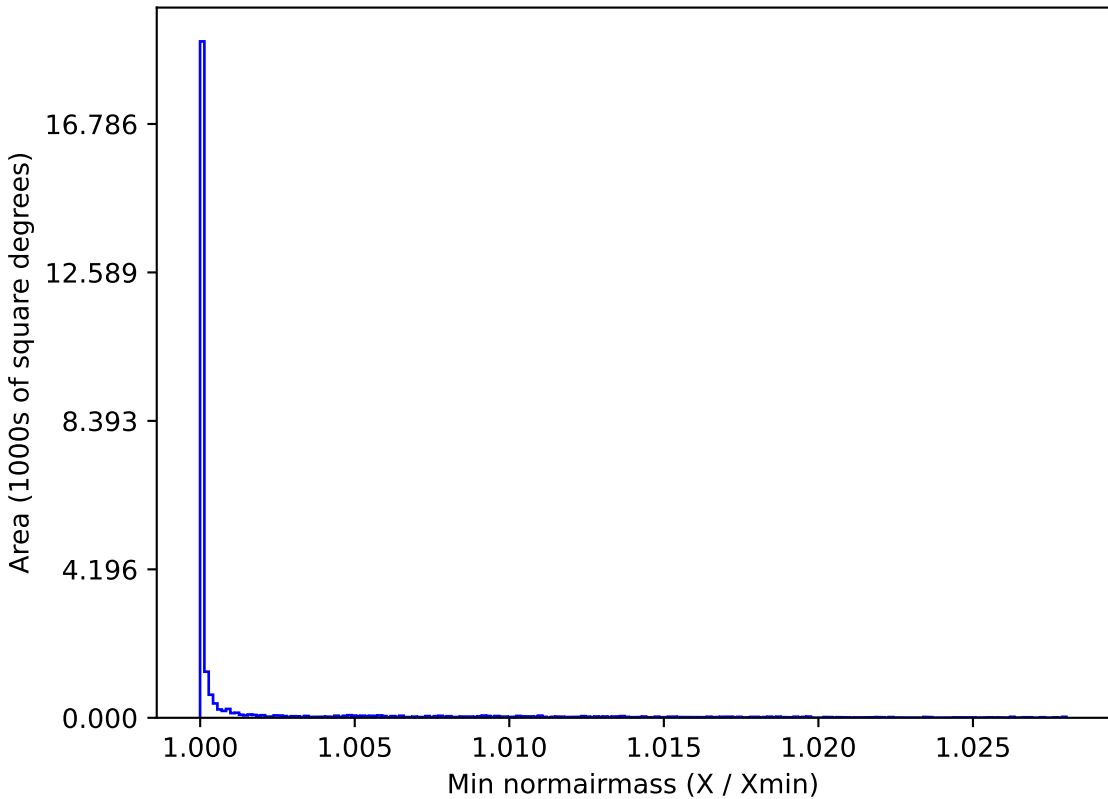
no_high_blob_v3.3_10yrs All sky z band: Min normairmass
