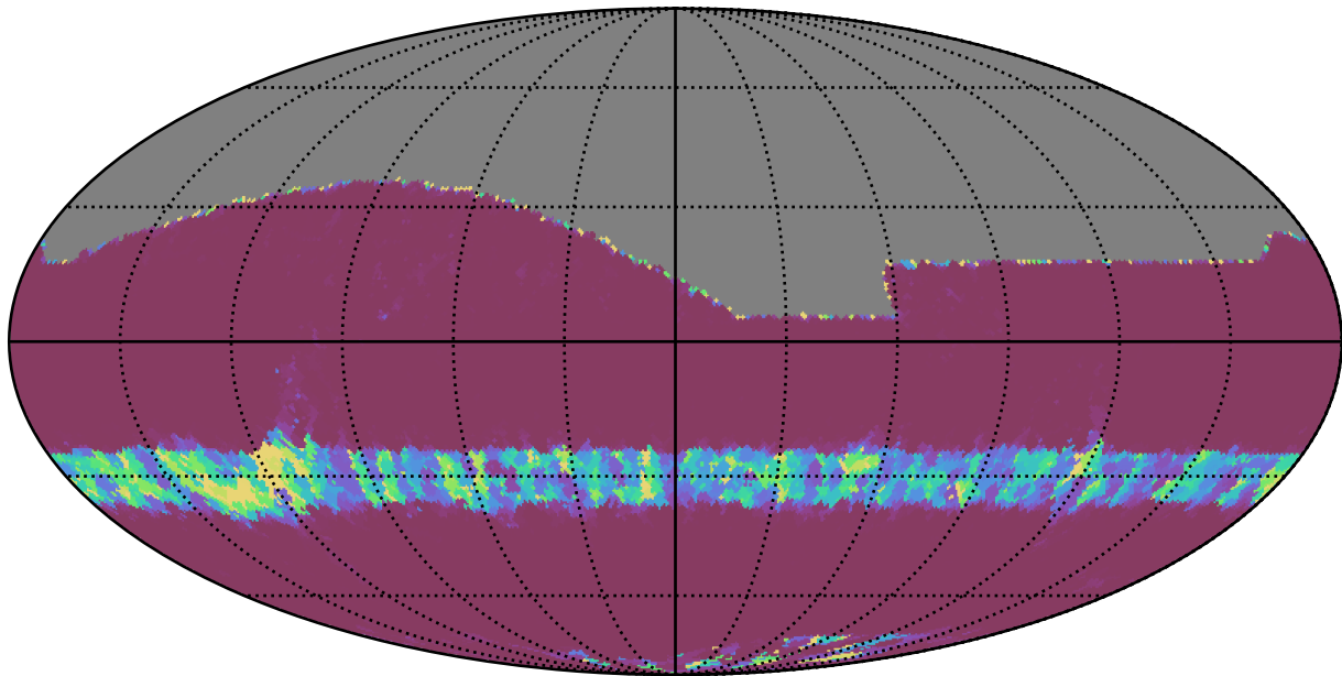
no_high_blob_v3.3_10yrs All sky r band: Min normairmass
