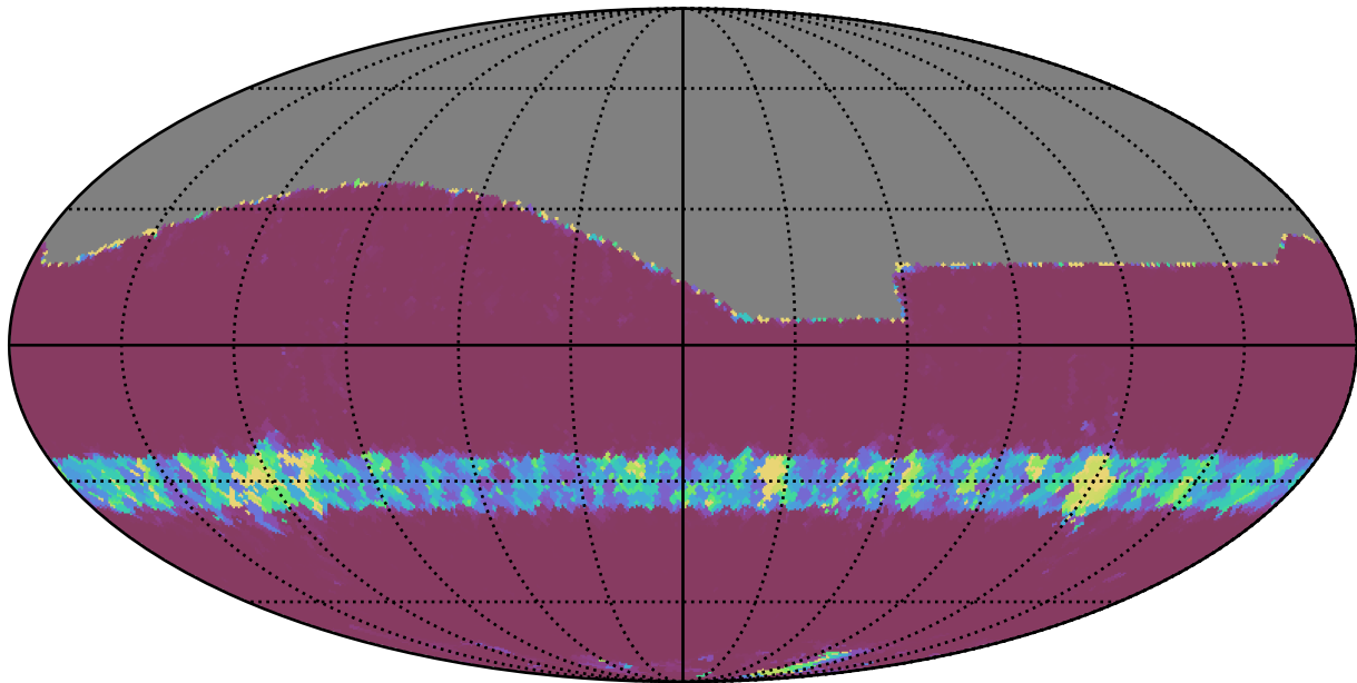
no_high_blob_v3.3_10yrs All sky i band: Min normairmass
