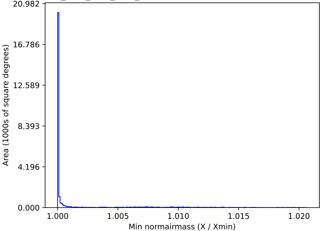
no_high_blob_v3.3_10yrs All sky i band: Min normairmass
