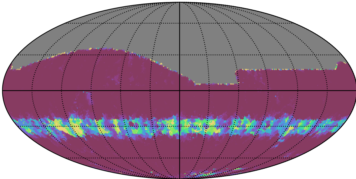
no_high_blob_v3.3_10yrs All sky g band: Min normairmass
