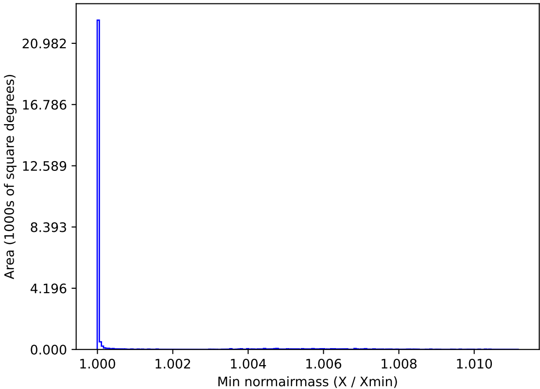
no_high_blob_v3.3_10yrs All sky all bands: Min normairmass
