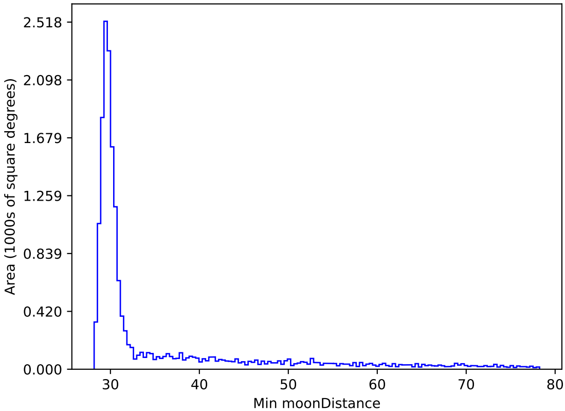
no_high_blob_v3.3_10yrs WFD z band: Min moonDistance
