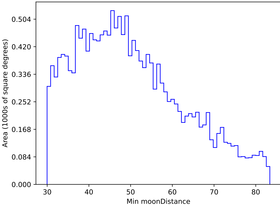
no_high_blob_v3.3_10yrs WFD u band: Min moonDistance
