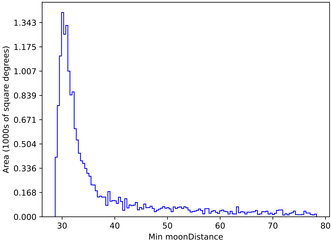
no_high_blob_v3.3_10yrs WFD r band: Min moonDistance
