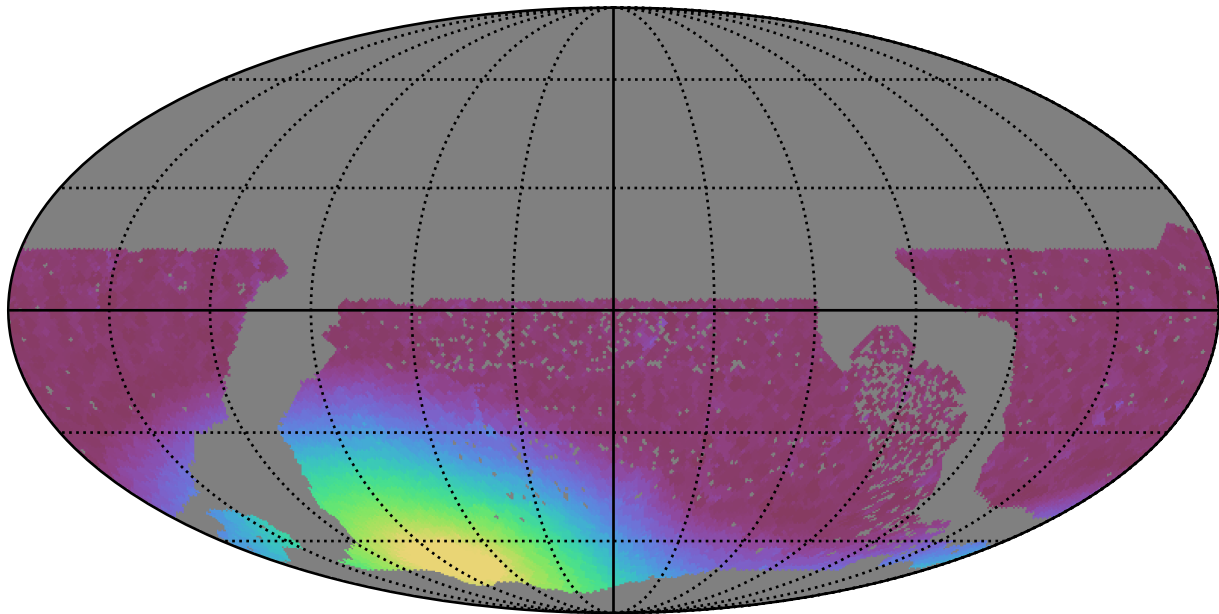
no_high_blob_v3.3_10yrs WFD i band: Min moonDistance
