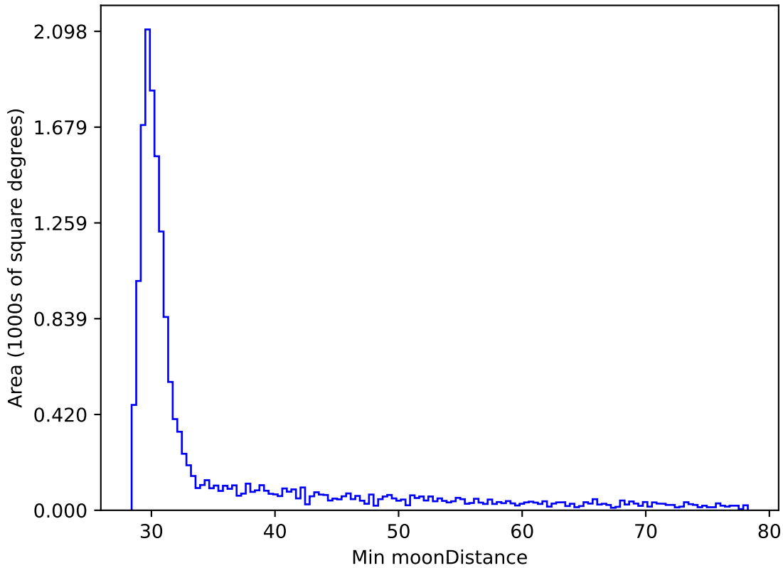
no_high_blob_v3.3_10yrs WFD i band: Min moonDistance
