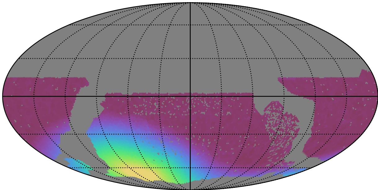
no_high_blob_v3.3_10yrs WFD all bands: Min moonDistance
