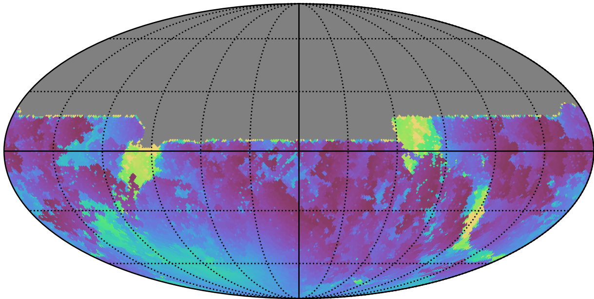
no_high_blob_v3.3_10yrs All sky u band: Min moonDistance
