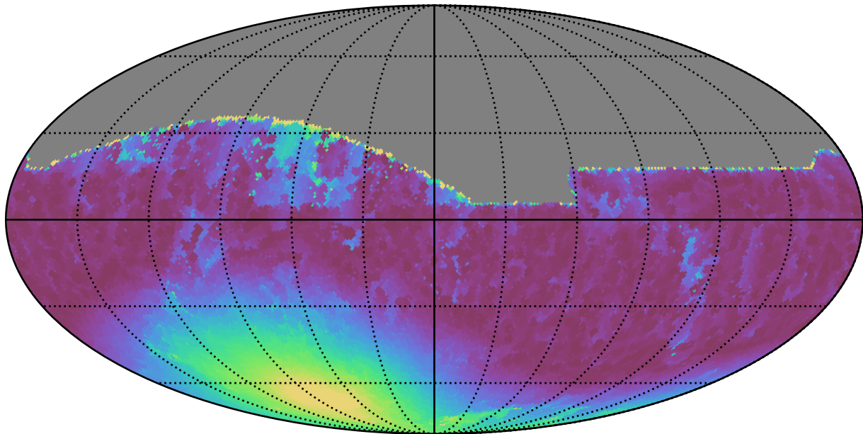
no_high_blob_v3.3_10yrs All sky r band: Min moonDistance
