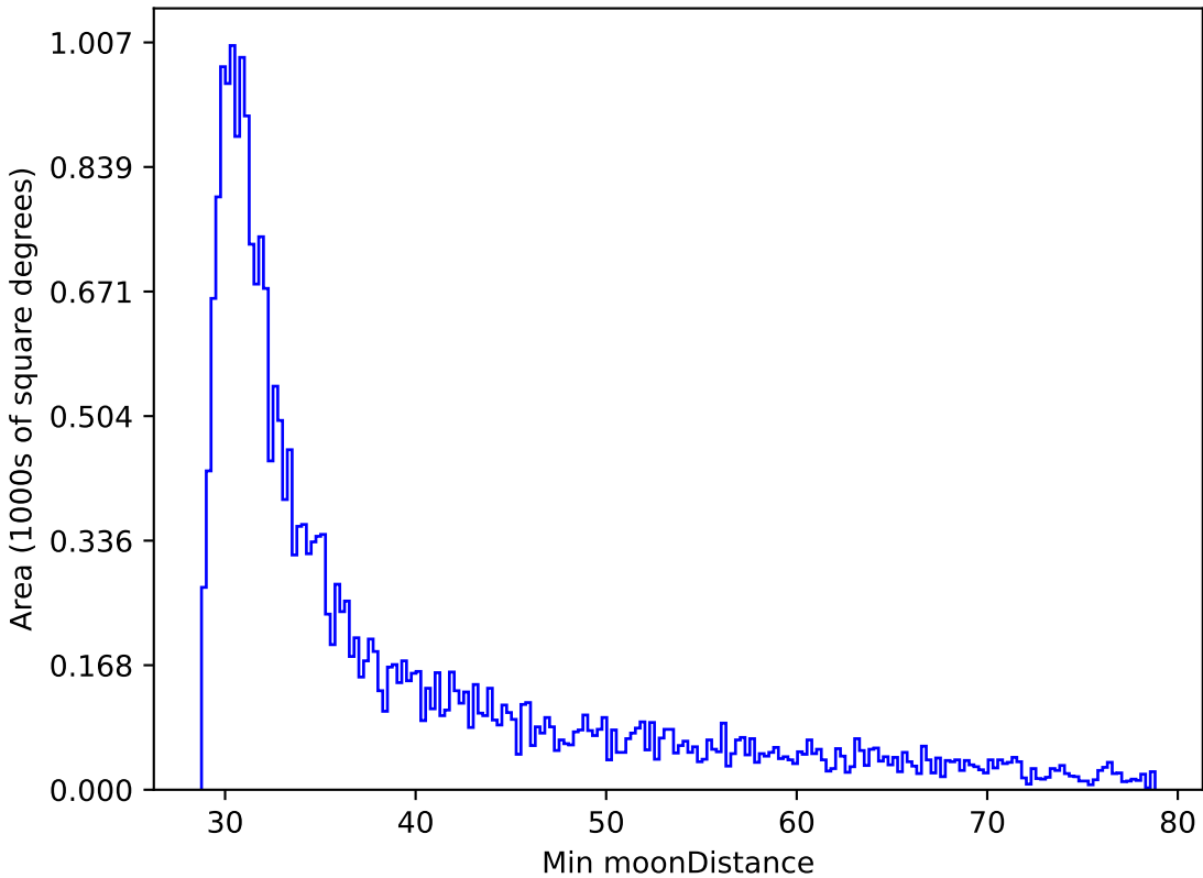
no_high_blob_v3.3_10yrs All sky r band: Min moonDistance
