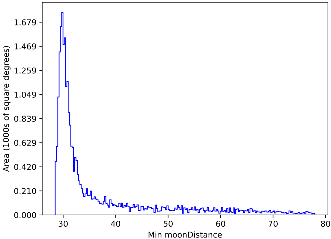
no_high_blob_v3.3_10yrs All sky i band: Min moonDistance
