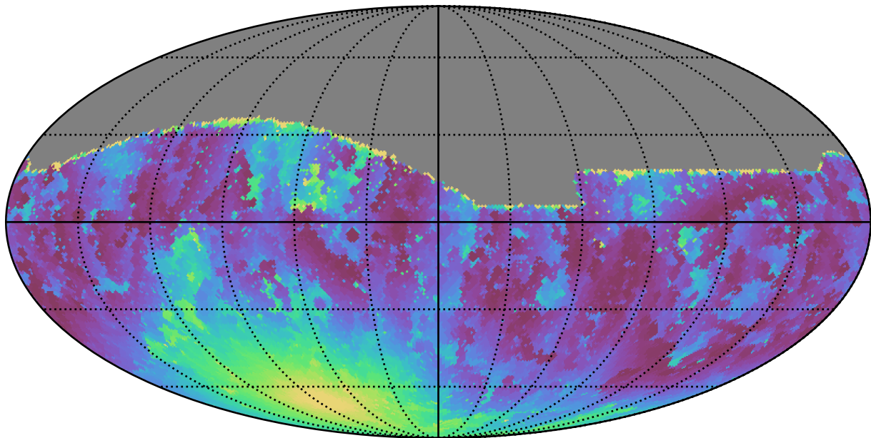
no_high_blob_v3.3_10yrs All sky g band: Min moonDistance
