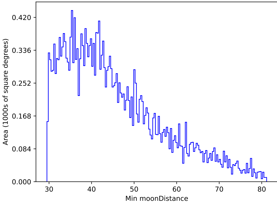
no_high_blob_v3.3_10yrs All sky g band: Min moonDistance
