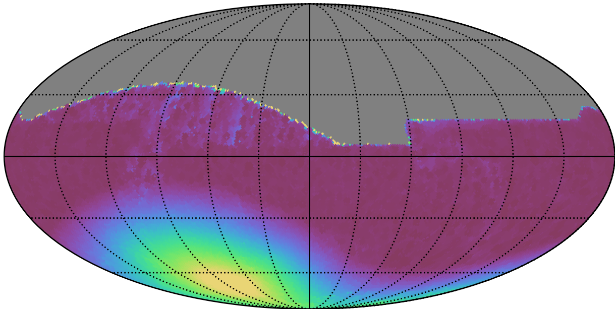
no_high_blob_v3.3_10yrs All sky all bands: Min moonDistance
