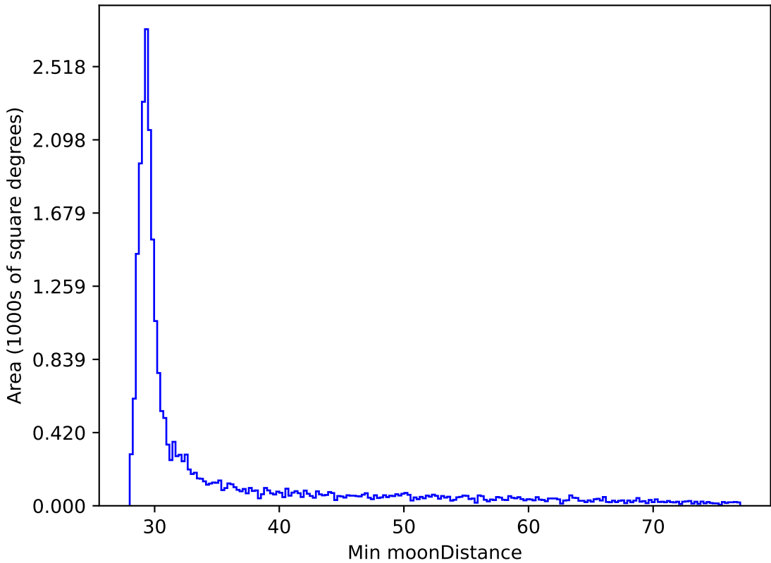
no_high_blob_v3.3_10yrs All sky all bands: Min moonDistance
