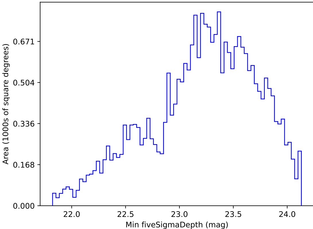
no_high_blob_v3.3_10yrs Yr 1 r band: Min fiveSigmaDepth
