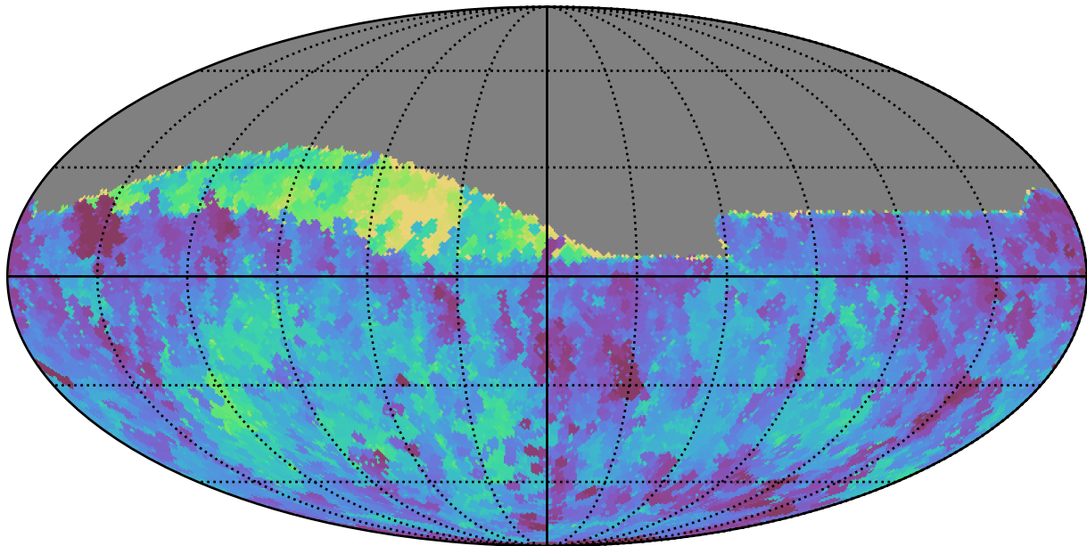
no_high_blob_v3.3_10yrs Yr 1 all bands: Min fiveSigmaDepth
