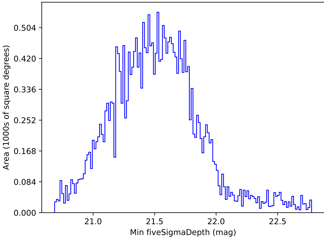
no_high_blob_v3.3_10yrs Yr 1 all bands: Min fiveSigmaDepth
