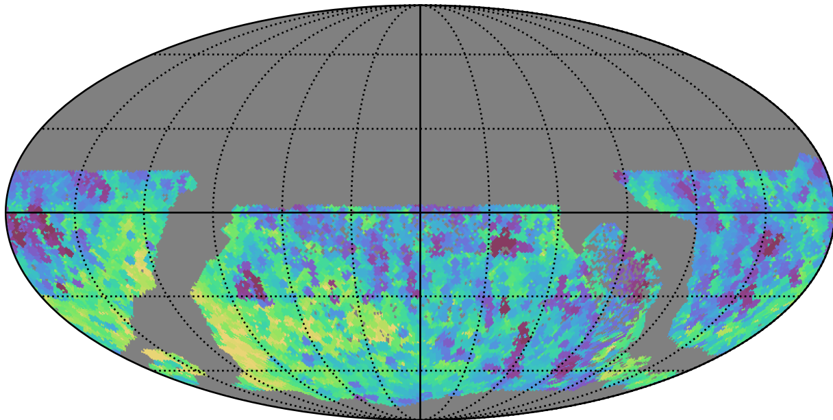
no_high_blob_v3.3_10yrs WFD all bands: Min fiveSigmaDepth
