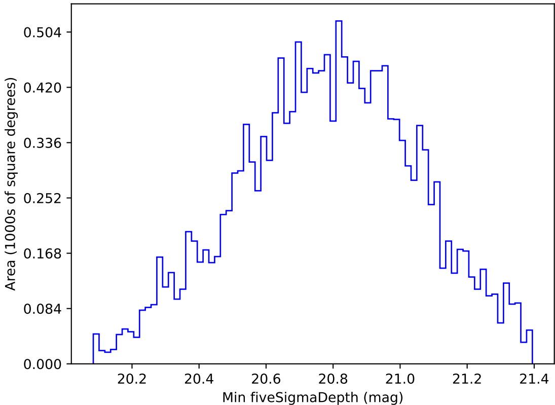
no_high_blob_v3.3_10yrs WFD all bands: Min fiveSigmaDepth
